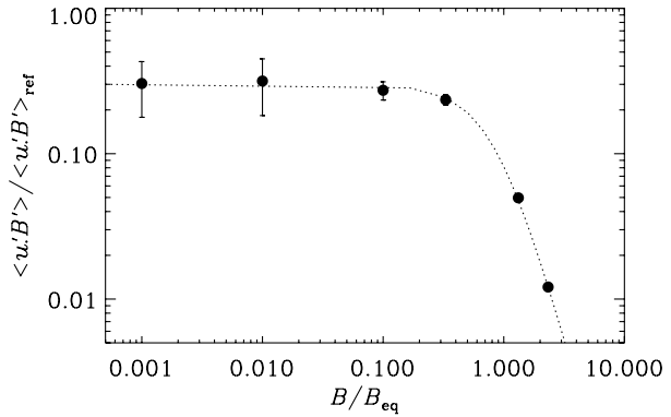
Figure 2 Dependence of the normalized cross helicity on the normalized vertical field strength for R_m = 10 , P_m = 1 , k_f/k_1 = 2.2 , and H_\rho k_1 = 2.5 . The dotted line corresponds to the graph of 0.3/[1 + (\langle \mathbf{B} \rangle / B_{\text{ref}})^2]^{3/2} with B_{\text{ref}} = 0.85 B_{\text{eq}} .
