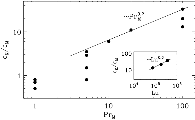
Fig. 12. Dependence of \epsilon_K/\epsilon_M on Pr_M . The solid line denotes 1.3 Pr_M^{0.7} , but many of the data points, predominantly those with smaller Lu , are beneath that line. The inset shows that for Pr_M = 100 , \epsilon_K/\epsilon_M increases with Lu like Lu^{0.6} .
