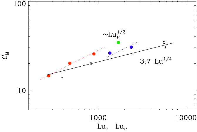
Fig. 5. Dependence of C_M on Lu and Lu_v . An approximate scaling \propto Lu^{1/4} is found for Lu < 6000 and a piecewise power-law scaling \propto Lu_v^{1/2} with different prefactors for the runs with higher viscosity ( 5 \times 10^{-6} red symbols and 4 \times 10^{-6} for the green symbol) and lower viscosity ( 2 \times 10^{-6} blue symbols).
