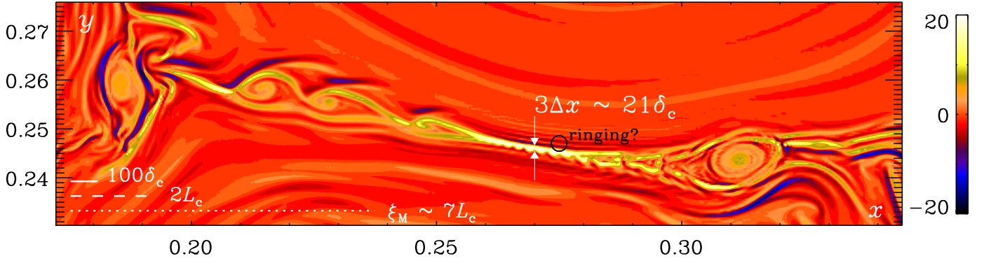
Fig. 14. Visualization of J_z(x, y) of Run 2m6 with \text{Pr}_M = 10 , \text{Lu} = 1.8 \times 10^5 , \text{Lu}_v \approx 5 \times 10^4 , and 16384^2 mesh points at t = 464 for a small part of the domain with sizes 2.8\xi_M(t) \times 0.74\xi_M(t) . The lengths of 100\delta_c , 2L_c , and \xi_M are indicated by horizontal white solid, dashed, and dotted lines, respectively. The thickness of the current sheet corresponds to about 3\Delta x \approx 21\delta_c . In its proximity, there are also indications of ringing, indicated by the black circle.
