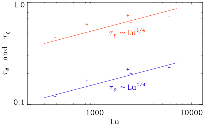
Fig. 8. Dependence of \tau_\varepsilon and \tau_\xi on Lu . The two show a similar dependence on Lu , approximately \propto Lu^{1/4} , but there is possible evidence for a leveling off for larger values of Lu .
