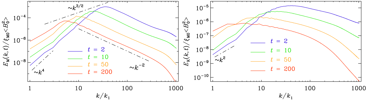
Fig. 3. Magnetic and kinetic energy spectra for Run M1 at different times. For large values of k there is a k^{-2} inertial range. The \propto k^4 and \propto k^2 slopes are indicated for reference. As elsewhere, time is in units of [t] = (c_s k_1)^{-1} .
