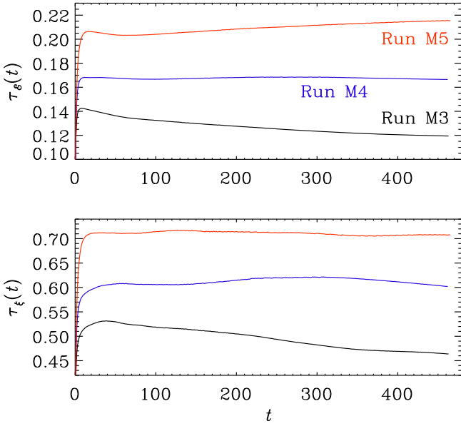
Fig. 7. Evolution of \tau_\varepsilon(t) and \tau_\xi(t) for three values of \text{Pr}_M with fixed and moderate viscosity. These times tend to be approximately constant at late times with values approximately consistent with those in Table 1.
