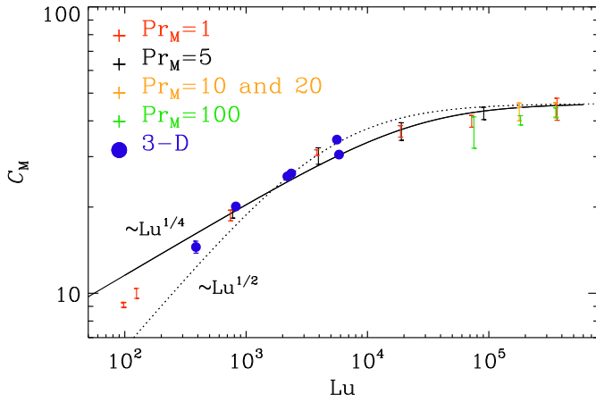
Fig. 13. Dependence of C_M on Lu for the 2D runs. Shallow scaling \propto Lu^{0.1} is found for 10^4 < Lu < 10^5 , which is also compatible with a leveling off at Lu_c = 2.5 \times 10^4 , as described by Eq. (24) with n = 1/4 . The black (red) data points are for Pr_M = 5 ( Pr_M = 1 ). The blue data points denote the 3D results from Sect. 4. The orange symbols are for the runs with Pr_M = 10 and 20 , listed in Table 3. The thin dotted line gives Eq. (24) with n = 1/4 for comparison.
