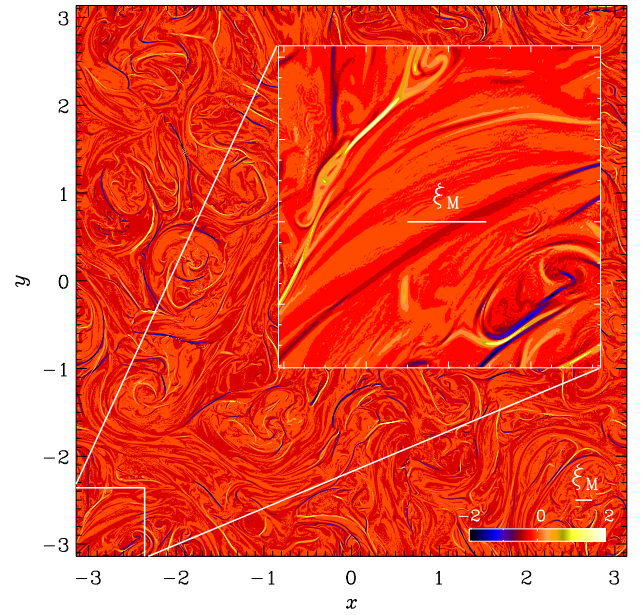
Fig. 2. Visualization of J_z at z = \pi along with a zoom-in on the lower left corner for Run M0, where \text{Pr}_M = 10 , at t = 644 . The value of \xi_M at that time is indicated by the length of the short white lines.
