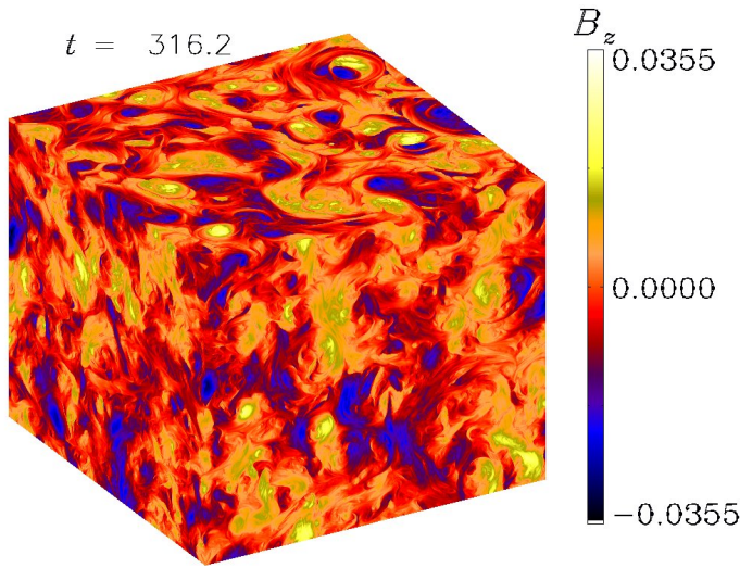
Fig. 1. Visualization of B_z on the periphery of the computational domain for Run M1, where \text{Pr}_M = 5 .
