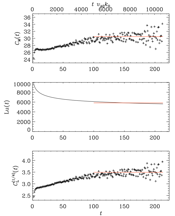
Fig. 4. Approach of C_M(t) , \text{Lu}(t) , and C_L^{(1/4)}(t) to an approximately constant value toward the end of the simulation for Run M1.
