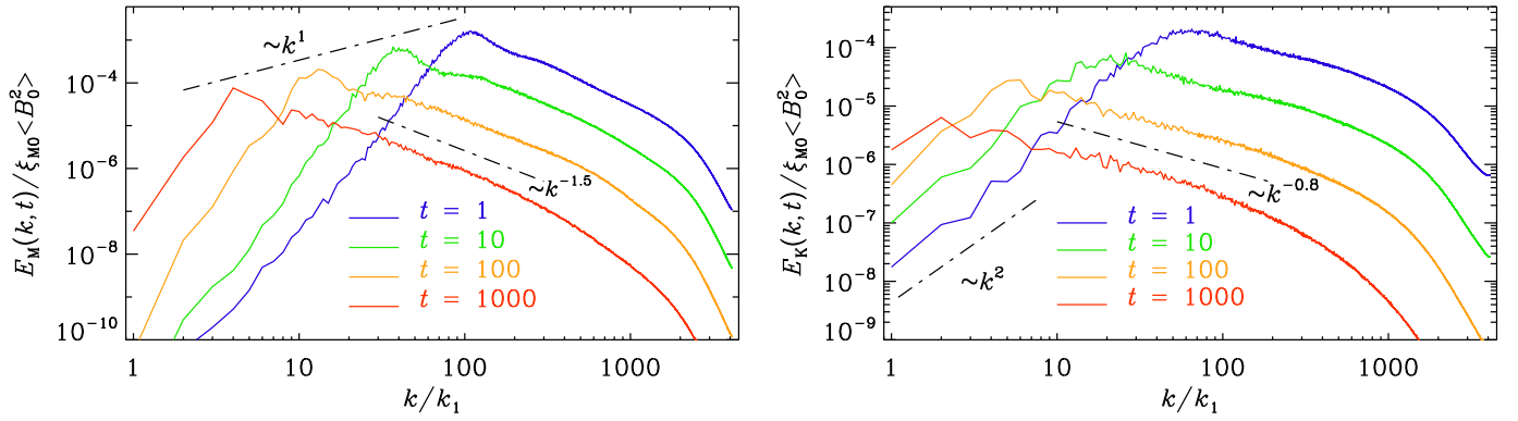
Fig. 10. Similar to Fig. 3, but for Run 2M1. The magnetic peaks lie underneath a k^\beta envelope with \beta = 1 , as expected in the case of anastrophy conservation.
