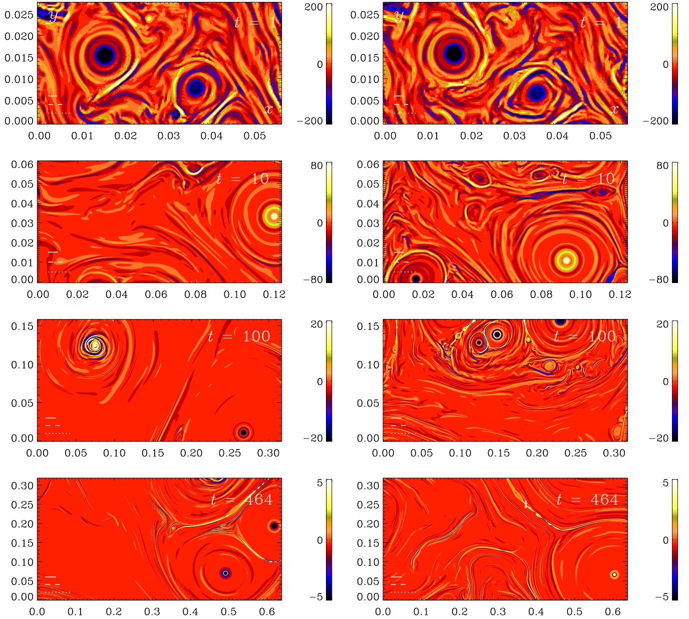
Fig. B.2. Similar to Fig. B.1, but for Run 2m1 with Lu = 75,000 (left) and Run 2m2 with Lu = 182,000 (right) using Pr_M = 100 and 16384^2 mesh points in both cases. The thick white line in the bottom right panel at (x, y) = (0.37, 0.25) marks the location of the cross section shown in Fig. 15.
