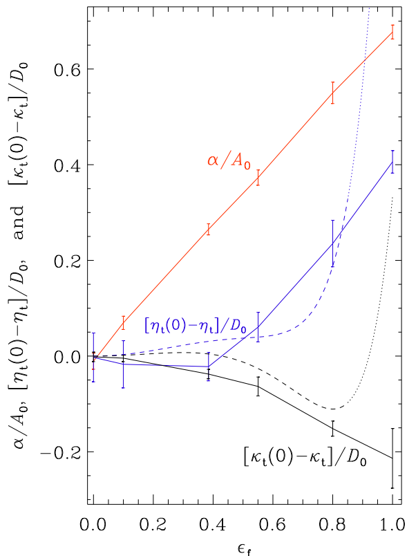
Figure 1. Dependencies of \alpha (red solid line), \eta_t(0) - \eta_t (blue solid line) and \kappa_t(0) - \kappa_t (black solid line) on the fraction \epsilon_f of the kinetic helicity, where \eta_t(0) = \eta_t(\epsilon_f = 0) and \kappa_t(0) = \kappa_t(\epsilon_f = 0) . Here \alpha is normalized by A_0 = u_{\text{rms}}/3 , and turbulent diffusion coefficients are normalized by D_0 = u_{\text{rms}}/3k_f , where k_f is the forcing wavenumber. The dashed blue and black curves give the expressions (1 + \epsilon_f^4)^3 \epsilon_f^2/3 - \epsilon_f^4 and (1 + \epsilon_f^4)^3 \epsilon_f^2/6 - \epsilon_f^4 from Equations (23) and (39), respectively. The theoretical results for \epsilon_f \gtrsim 0.85 are shown as dotted lines, because they may not be reliable.
